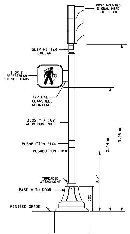
PEDESTAL MOUNTING
