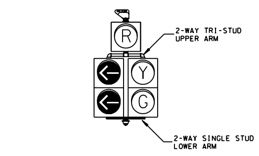
5-SECTION SIGNAL HEAD
