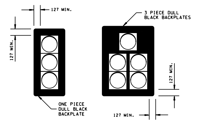
TRAFFIC SIGNAL BACKPLATE DETAIL
