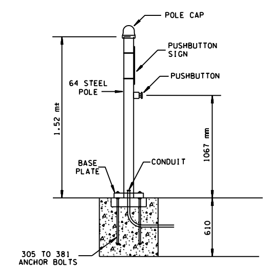
PEDESTRIAN PUSHBUTTON POST
