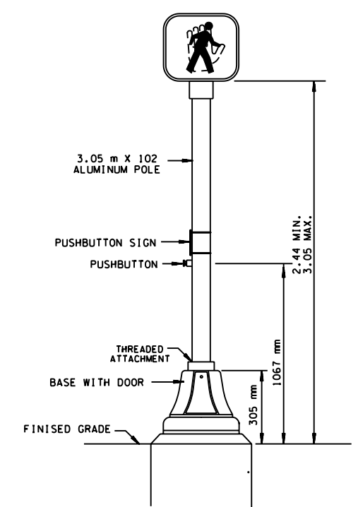
PEDESTAL MOUNTING
