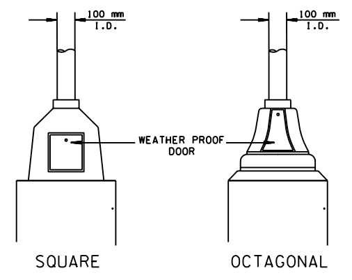
CAST PEDESTAL BASE ALTERNATES
