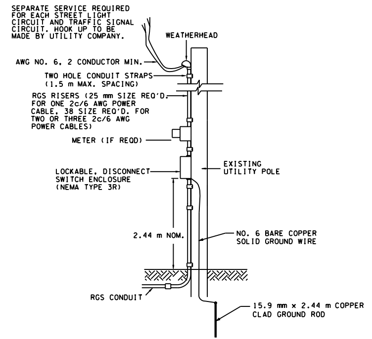
POWER SERVICE DETAIL
