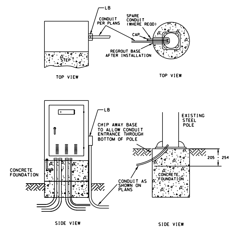
CONDUIT ENTRANCE DETAIL (EXISTING CABINET OR POLE)
